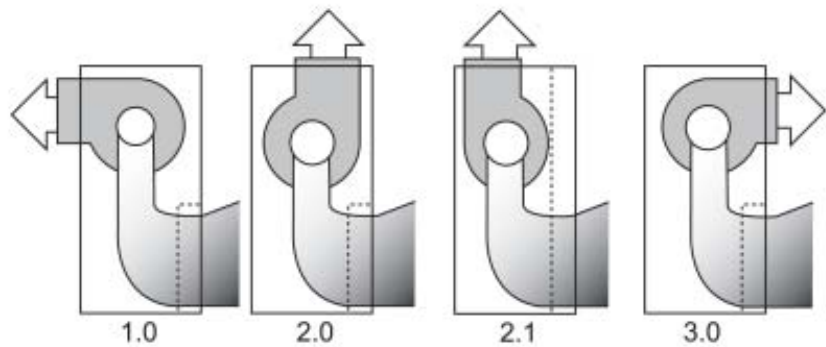
Figure 1 - Fan arrangement
